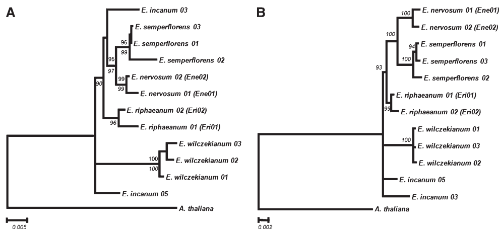
Fig. 5. Phylogenetic position of Erysimum nervosum and E. riphaeanum populations within the North African species of the genus Erysimum . (A) Maximum likelihood tree obtained with PhyML; branch reliability supports, calculated by approximate likelihood ratio test, appear below branch lines, and bootstrap values above branch lines. (B) Tree obtained using Bayesian Markov chain Monte Carlo inference; branch supports values are posterior probabilities. Only branch supports higher than 75% are shown.
